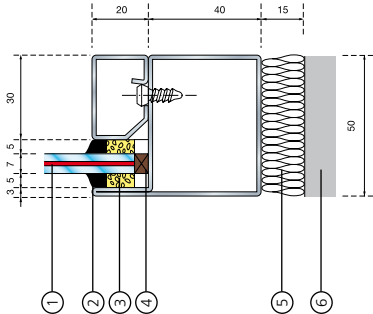
P.V. 96-A-324 Profil Jansen Economy 50
